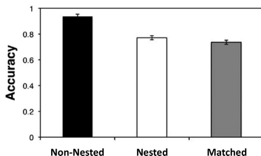
Figure 3. Judgment accuracy as a function of task and evidence in Experiment 1. Error bars represent one standard error.
