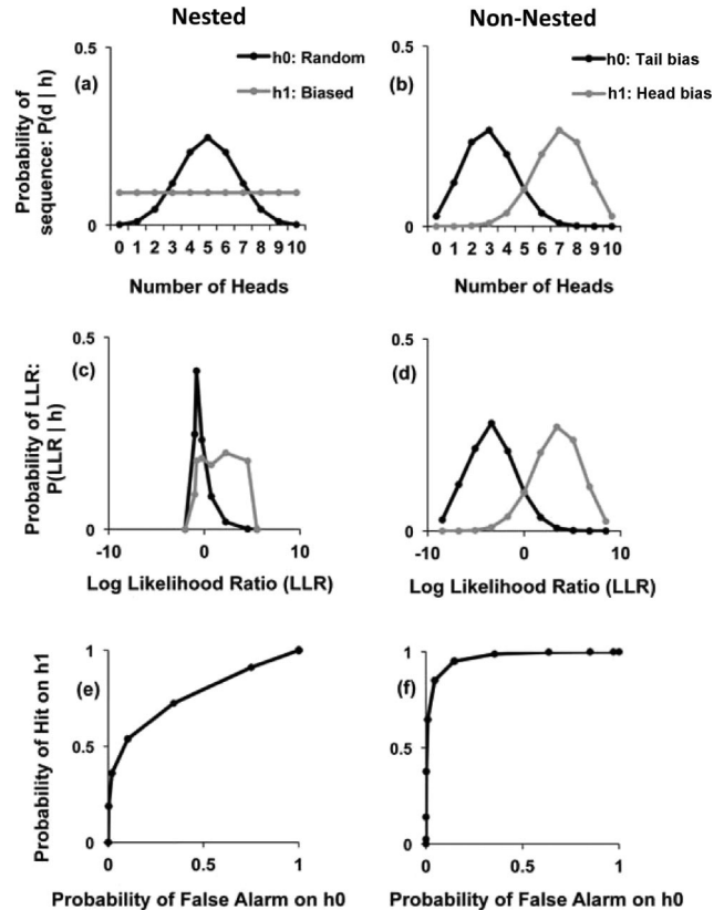
Figure 1. The statistical challenge posed by randomness detection. The left column shows model predictions for the nested problem of randomness judgment: discriminating whether events like head/tail flips or repetition/alternation of flips are equiprobable or systematically biased. The right column shows the model predictions for the non-nested problem of discriminating the direction of systematic bias. Plots show the probability distribution over sequences for (a) nested and (b) non-nested hypotheses, the distribution of evidence (measured by the log likelihood ratio or LLR) for each of the (c) nested and (d) non-nested hypotheses, and the receiver operating characteristic curves produced by a signal detection analysis for the (e) nested and (f) non-nested discrimination tasks.
