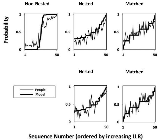
Figure 9. Experiments 3A (top three panels) and 3B (bottom two panels): Proportion of people reporting that a sequence was generated by h_1 , and posterior probability of h_1 under the model. h_1 represented a sequentially dependent process biased to repeat or alternate for the nested condition, and a bias to repeat flips for the symmetric and matched conditions. Sequences are ordered by increasing evidence for h_1 . LLR = log likelihood ratio.
