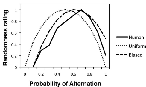
Figure 7. Human and model randomness ratings for binary sequences presented by Falk and Konold (1997). The uniform model assumes that repetitions and alternations are judged equally systematic, whereas the biased model assumes that repetitions are more systematic than alternations.
