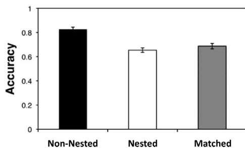
Figure 10. Judgment accuracy as a function of task and evidence in Experiment 3B. Error bars represent one standard error.
