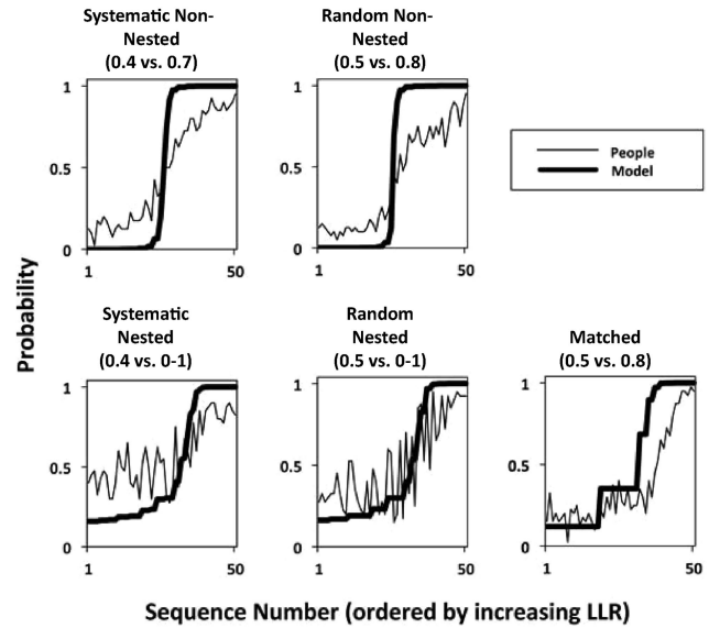
Figure 6. Results of Experiment 2, showing the proportion of people reporting that a sequence was generated by h_1 and posterior probability of h_1 under the model. h_1 represented a systematically biased process for the nested conditions and a bias to heads for the symmetric and matched conditions. Sequences are ordered by increasing evidence for h_1 . LLR = log likelihood ratio.
