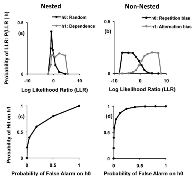
Figure 2. An alternative pair of non-nested hypotheses. The left column replicates the nested model from Figure 1. The right column shows the non-nested model where systematic processes are distributed over intervals 0 to 0.5 and 0.5 to 1. Plots show the distributions of the log likelihood ratio (LLR) for these (a) nested and (b) non-nested processes, and receiver operating characteristic curves for discriminating (c) nested and (d) non-nested processes.
