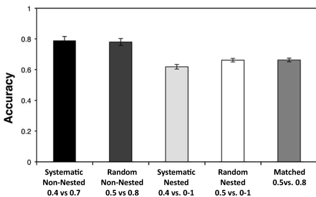
Figure 5. Judgment accuracy as a function of task and evidence in Experiment 2. Error bars represent one standard error.
