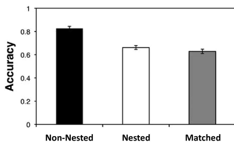
Figure 8. Judgment accuracy as a function of task and evidence in Experiment 3A. Error bars represent one standard error.
